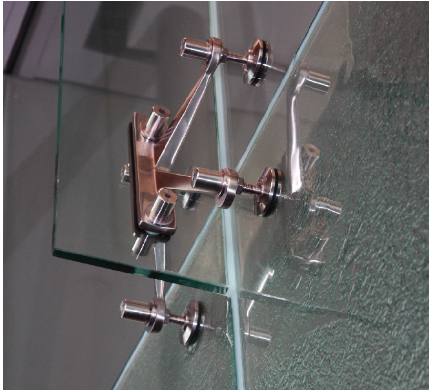
Texture:MD216 Fissure 1/2" Clear Tempered Kiln-Fired Glass
